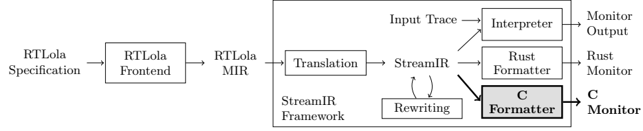
Fig. 2: Overview of the StreamIR framework
